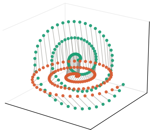
Spiral
