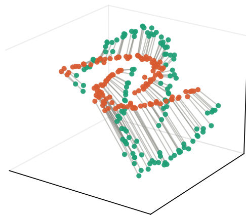
Two Moons
