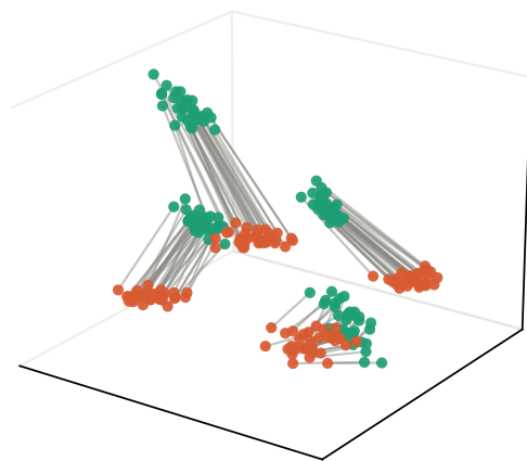
GMM
