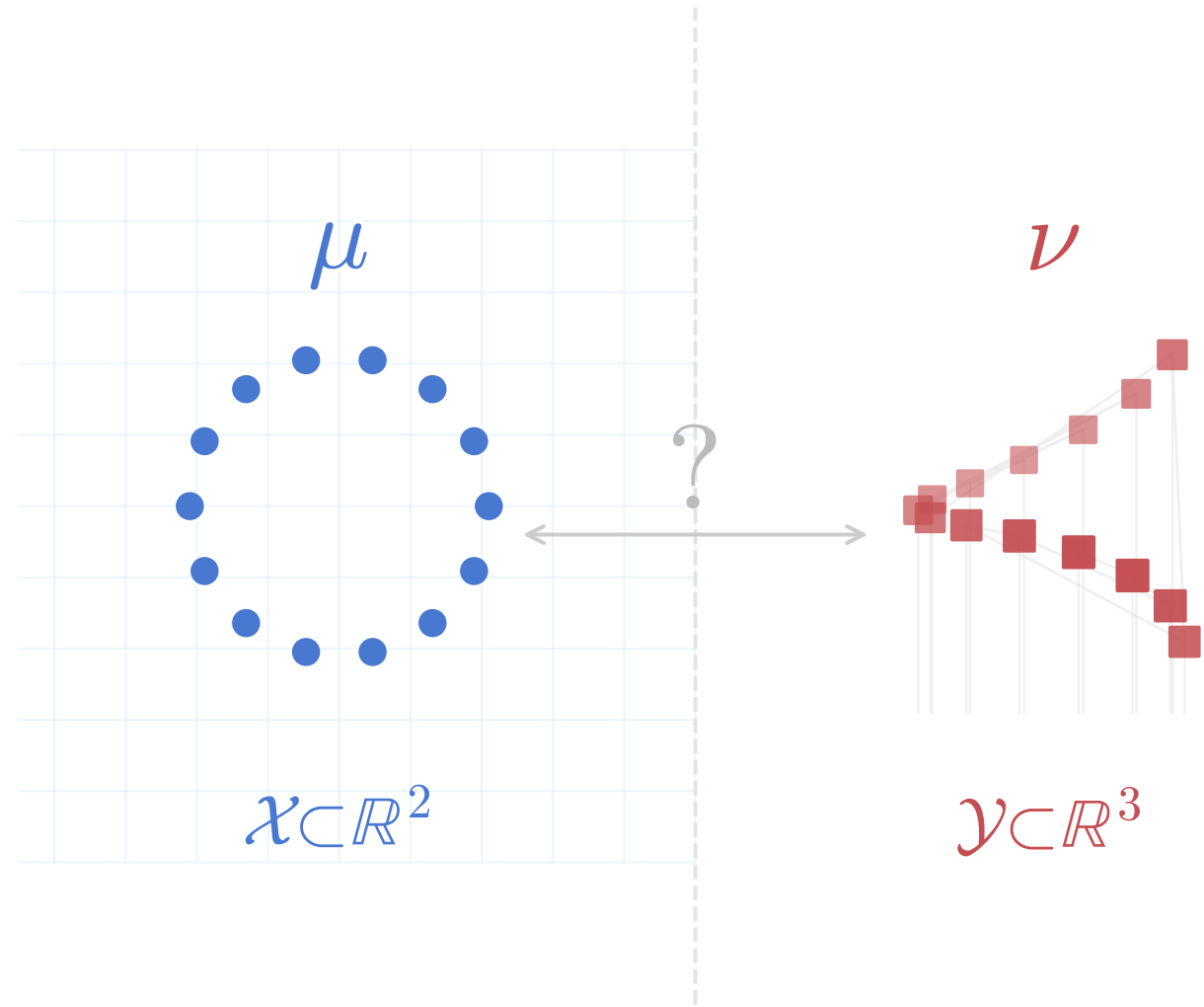
(a) Two metric spaces
